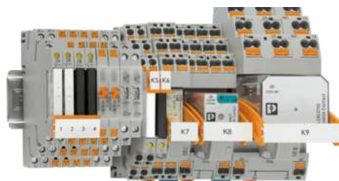
Solid-state relays and electromechanical relays
