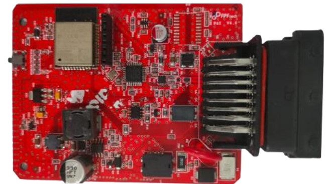
Automotive – Main Controller Card
