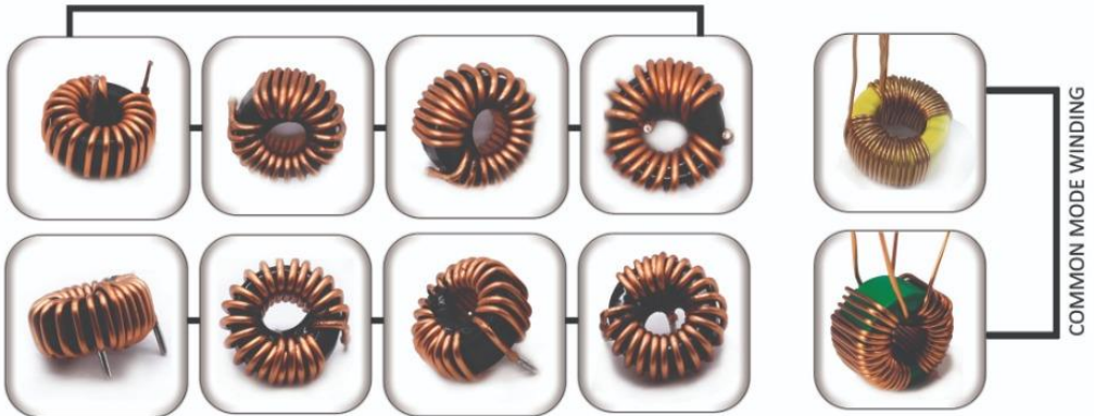
FULL COIL WINDING
